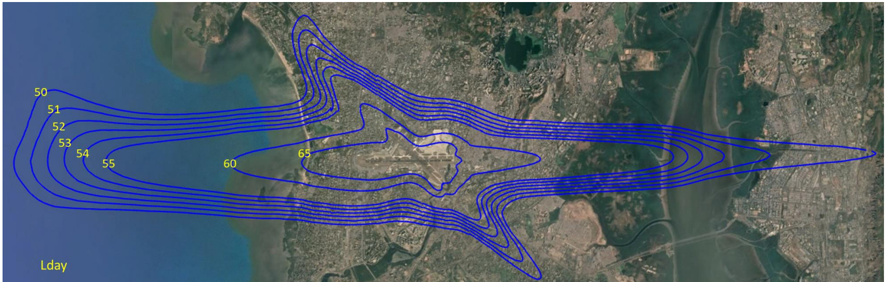
Figure-10 : Noise contours for Lday 50 to 65 dBA
